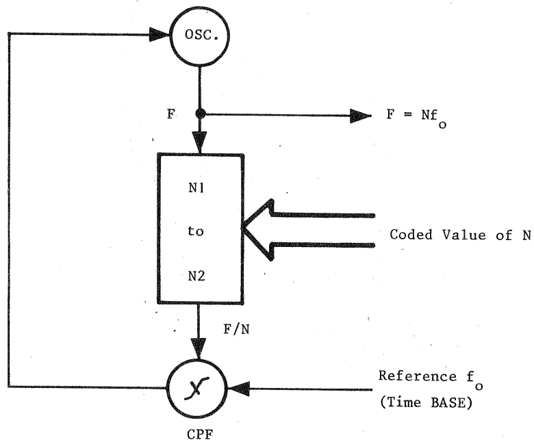
FIGURE VI-1 - Frequency synthesis
